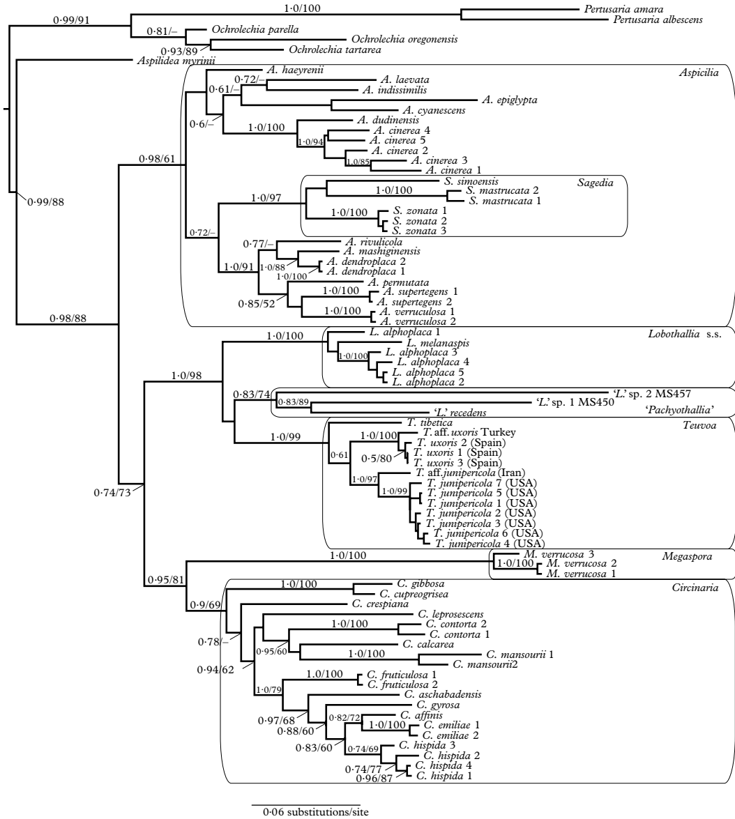
FIG. 1. Phylogenetic relationships within Megasporaceae , including the new genus Teuvoa , derived from Bayesian inference of nuclear ribosomal ITS and LSU sequence data. Values at each node indicate non-parametric bootstrap support (BS)/posterior probability (PP). Only support indices \geq PP 0.50/BS 50 are indicated. With the exception of the newly described genus in this study, Teuvoa , generic concepts within Megasporaceae follow Nordin et al. (2010) and Sohrabi et al. (2012).
